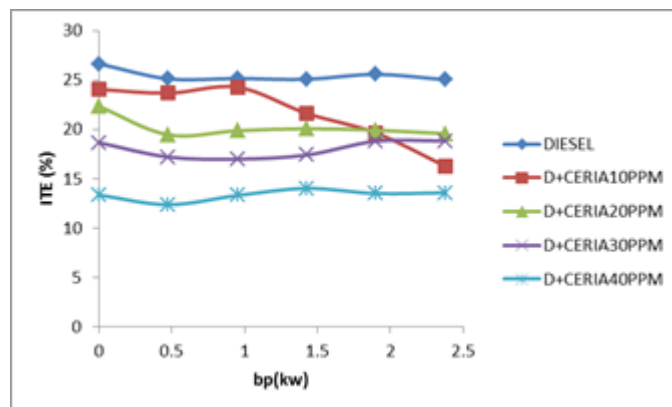
Fig.7. Variation of indicated thermal efficiency with brake power
