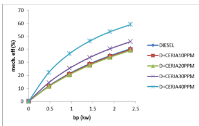
Fig.6. Variation of mechanical efficiency with brake power
