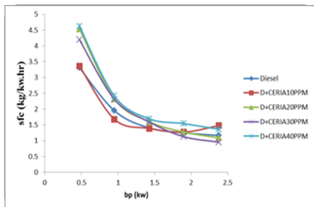
Fig.5. Variation of specific fuel consumption with brake power
