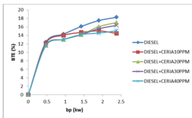
Fig.8. Variation of brake thermal efficiency with brake power
